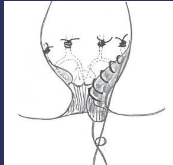
RAR = mucopexie
